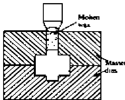
Fig 1.70 Investment casting
