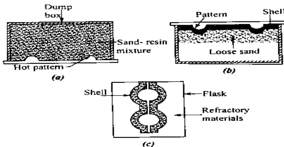
Fig 1.69 Shell moulding
