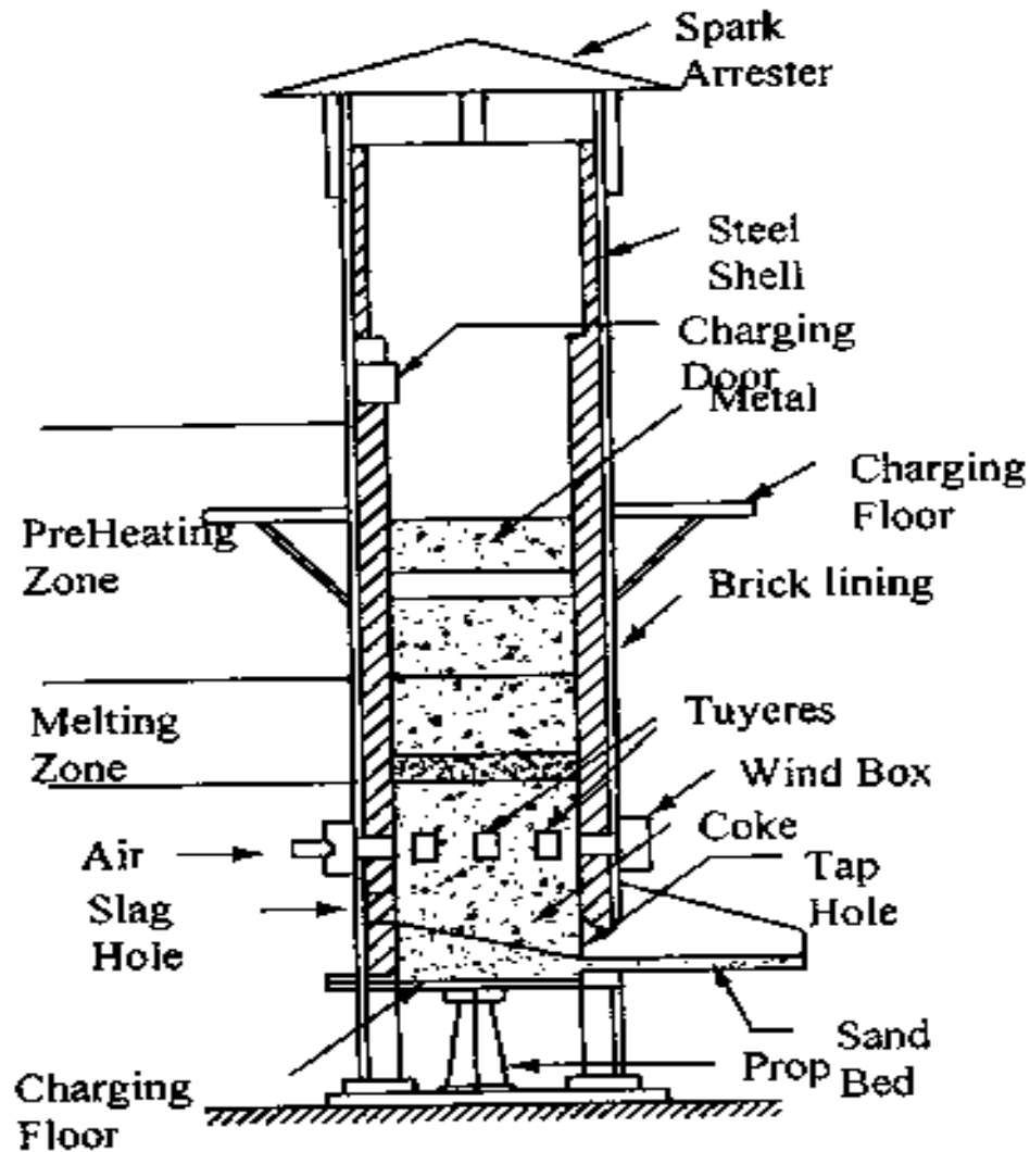
Fig 1.62 Cupola furnace
