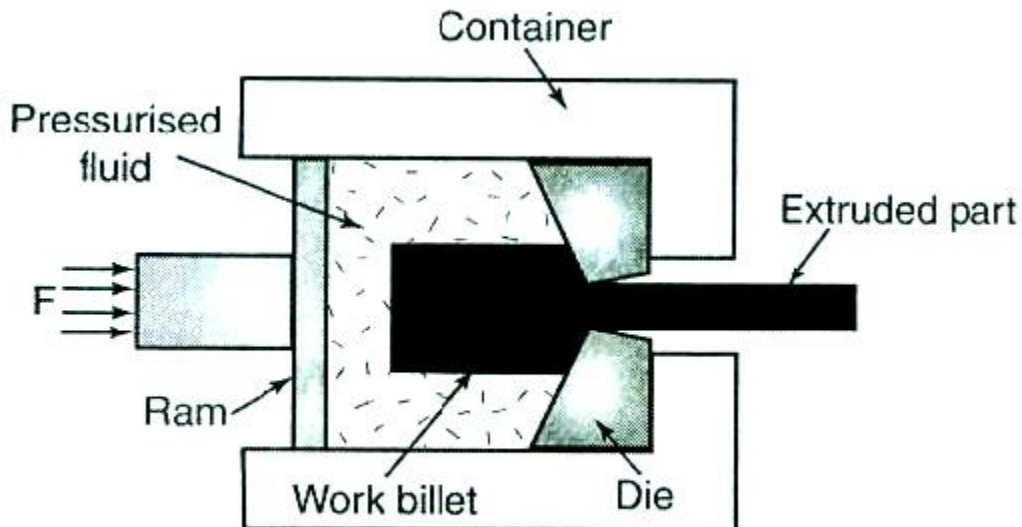
Figure: Hydrostatic extrusion
