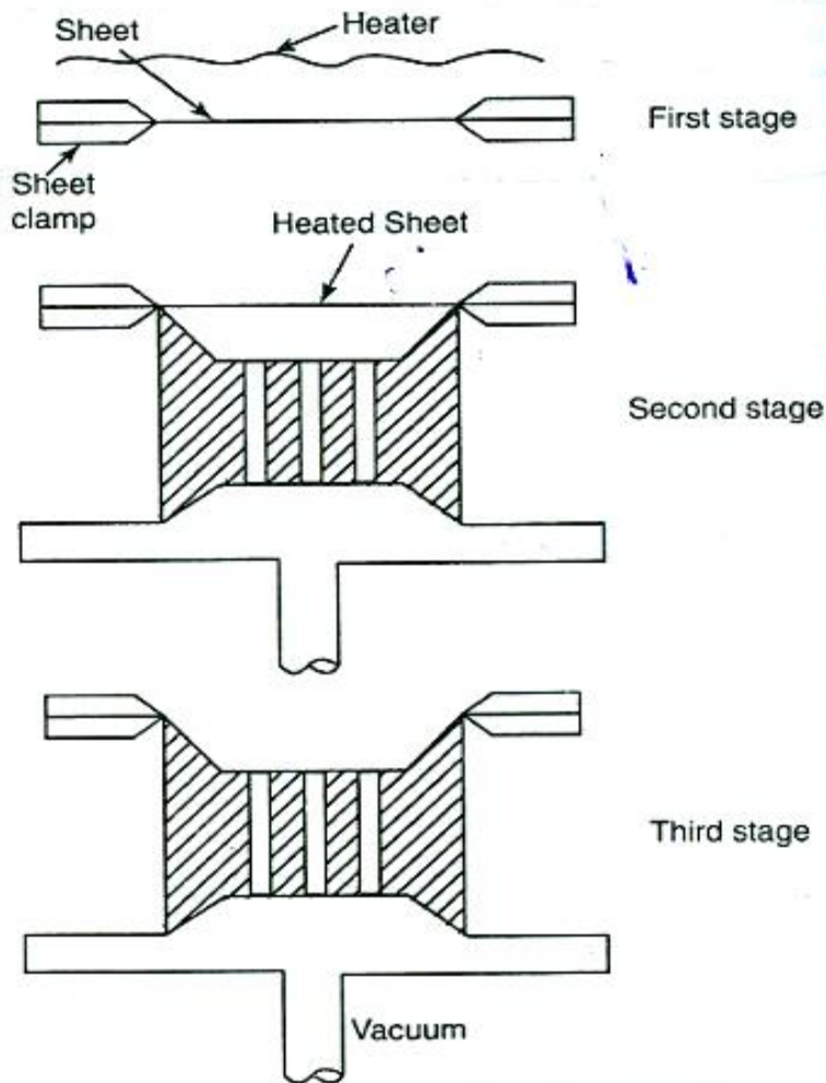
Fig. 5.8. Thermo forming stages
