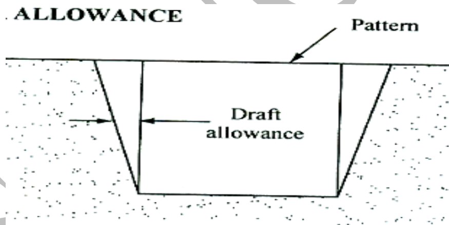
Fig 1.10 Draft allowance
